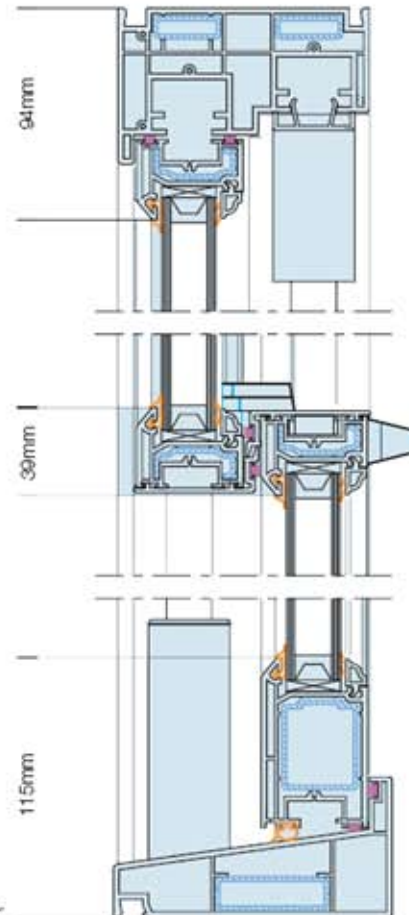
Vertical Section
